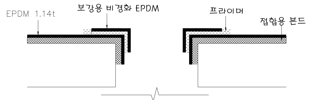
Drain Detail none scale
