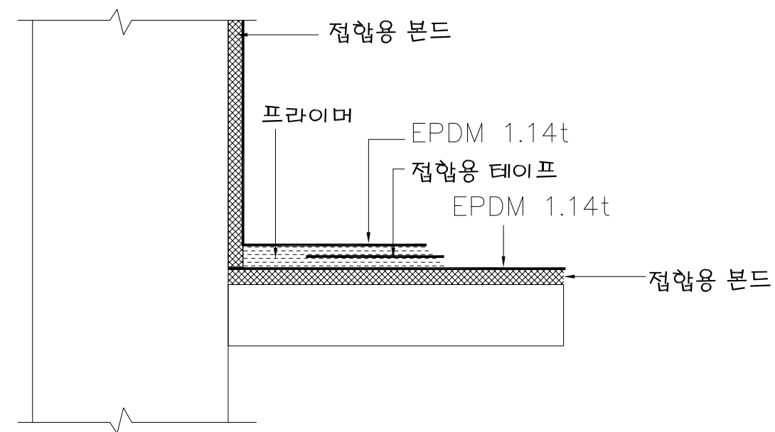
Corner none scale
