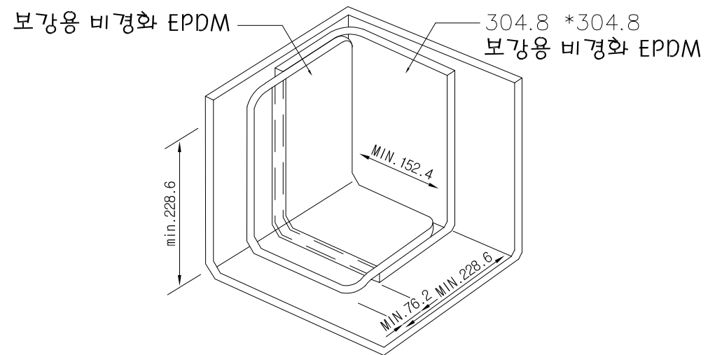
Incorner Detail none scale
