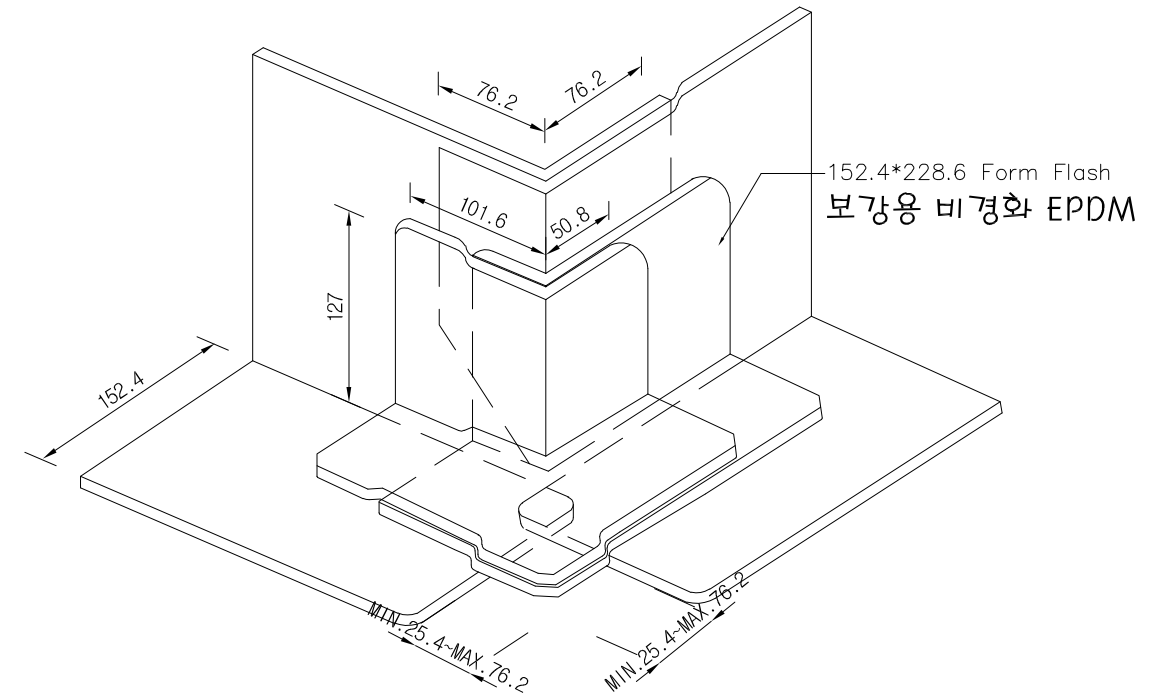
Outcorner Detail none scale
