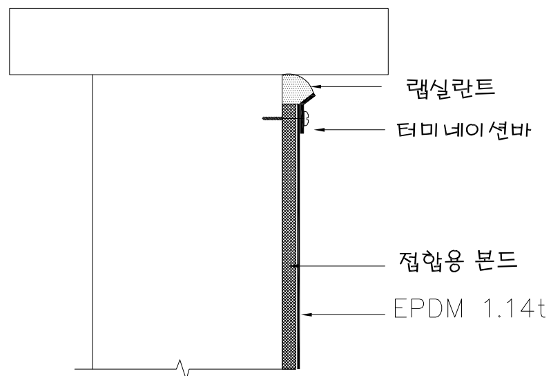
Termination Bar none scale
